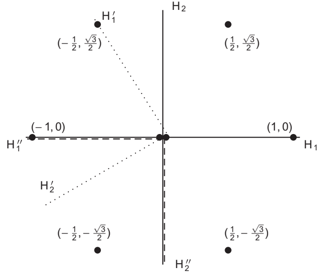
Figure 4. Root system of SU(3). The axes H_1 and H_2 show the angles that the root vectors make with respect to the two elements of the Cartan subalgebra. The primed and double primed axes represent two other equivalent sets of axes, one corresponding to the center of the group SU(3) and the other to the group SU(2).
