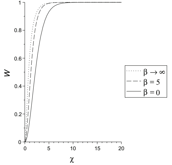
Figure 1. Shown are numerical solutions of the function w(x) when \beta = 5 and \beta \rightarrow \infty . For comparison the exact solution when \beta = 0 is also shown.
