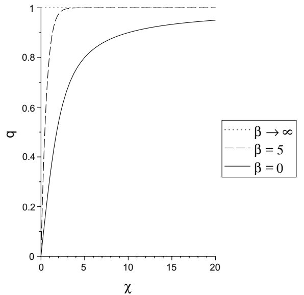
Figure 2. Shown are numerical solutions of the function q(x) when \beta = 5 and \beta \rightarrow \infty . For comparison the exact solution when \beta = 0 is also shown.
